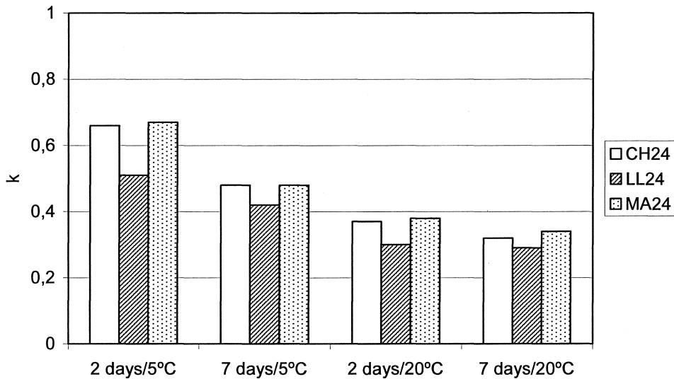
FIGURE 13 k -values for different curing conditions for filler produced from chalk, limestone or marble. Paste with 24% filler content.
