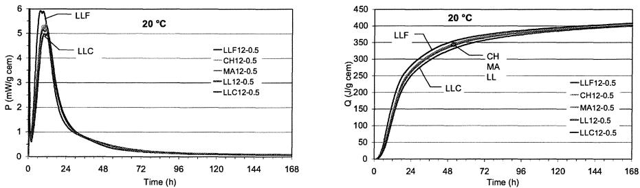
FIGURE 3 Heat production rate and heat per gram cement at 20^{\circ}\text{C} . Mixtures with 12% filler and W/B 0.5. Comparison between marble, chalk and coarse, medium or fine limestone.
