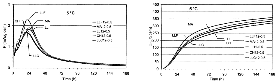
FIGURE 2 Heat production rate and heat per gram cement at 5^{\circ}\text{C} . Mixtures with 12% filler and W/B 0.5. Comparison between marble, chalk and coarse, medium or fine limestone.
