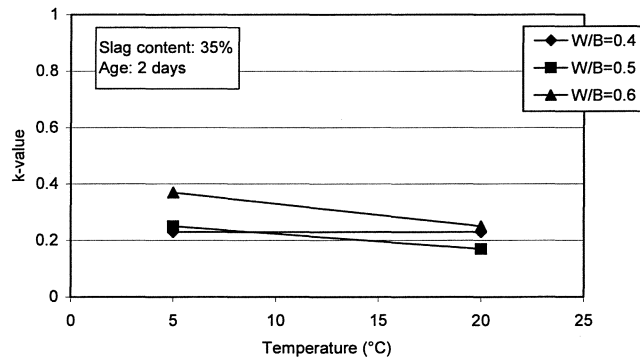
Fig. 5. The k -value for mortar containing slag, as a function of temperature. 2-days old mixtures.
